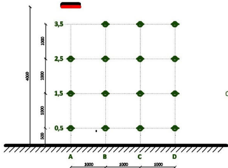
Figure 2-1 Scheme of measuring mesh under tested panel
